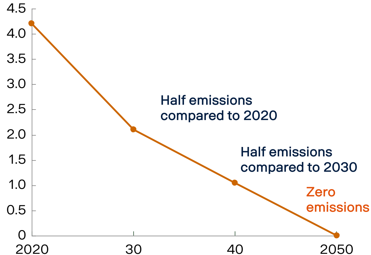
The global carbon law applied to transport* GtCO 2 /yr
